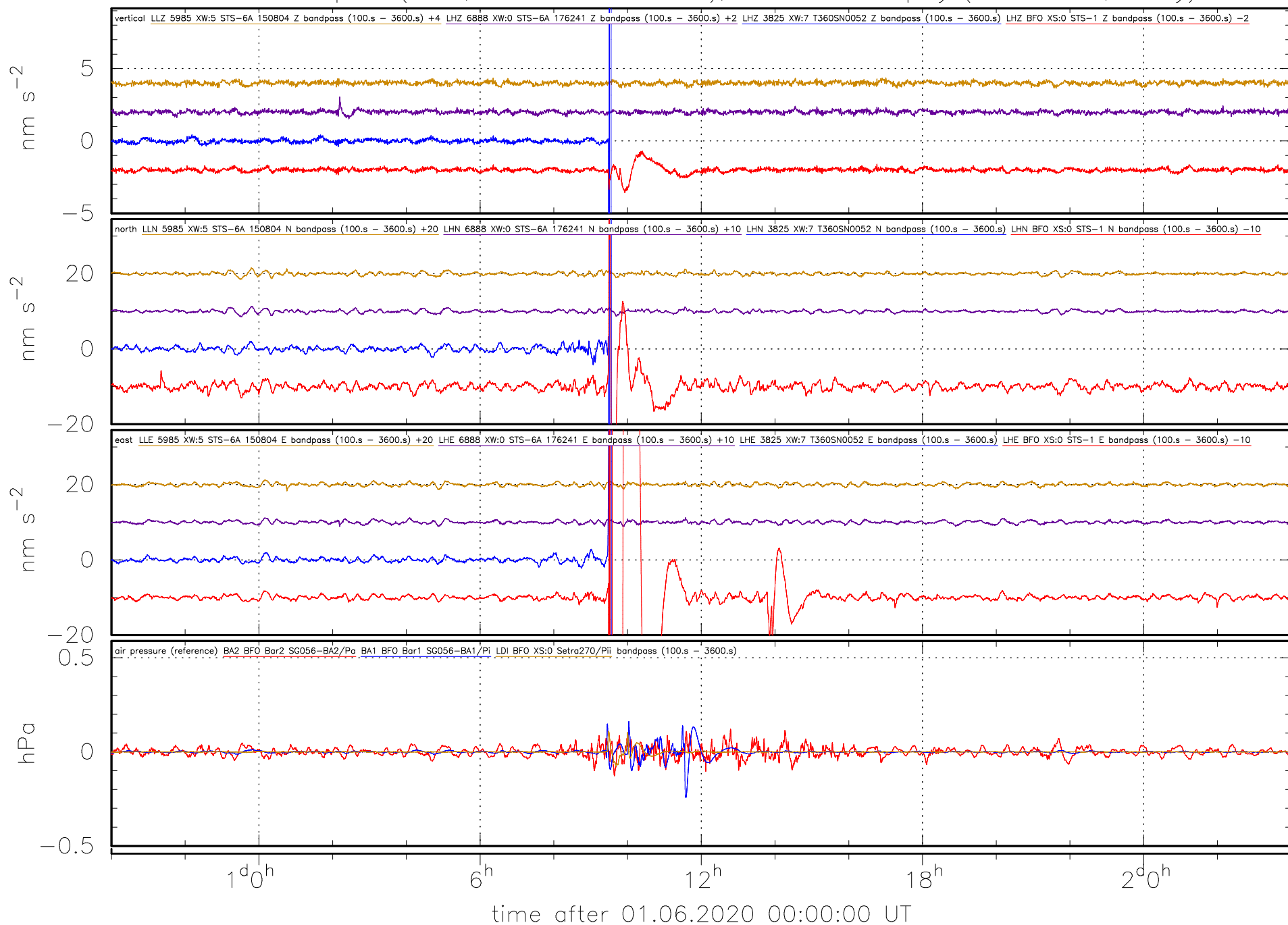
Normal mode bandpass (T360, STS-6A and STS-1), fixed scale display (02.06.2020, 1 day)
