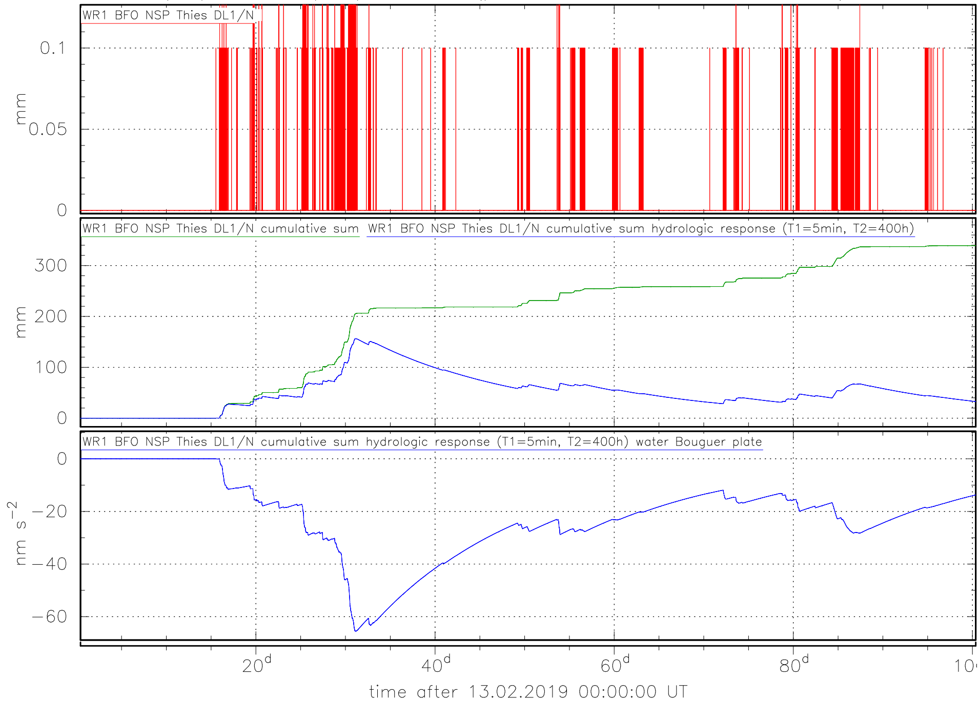
Thies DL1/N pluviometer: precipitation data (plot created at 24.05.2019 09:59:53 UT)
