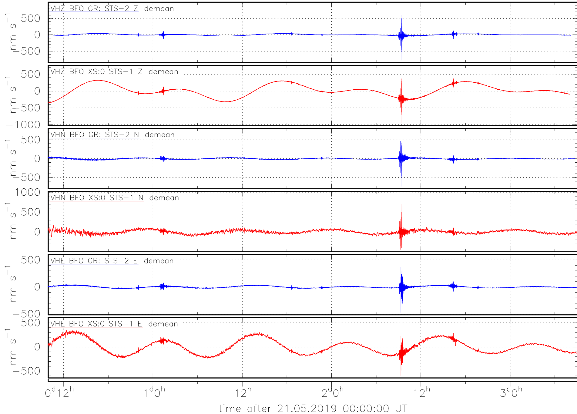
Seismometers long period data (raw data; units valid in passband only) (plot created at 24.05.2019 09:55:39 UT)
