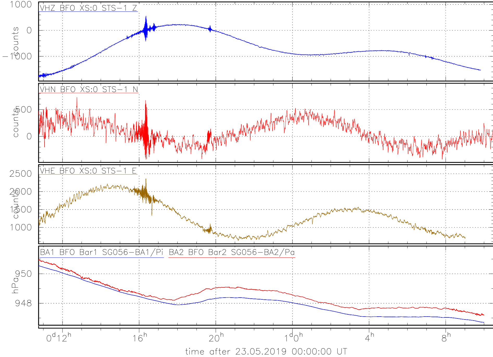
STS-1 VLP data (plot created at 24.05.2019 10:45:10 UT)
