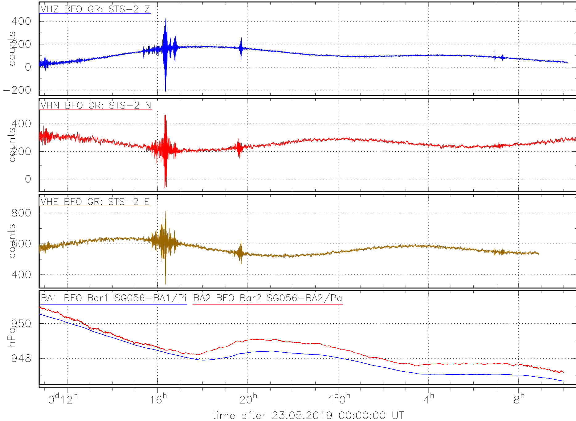
STS-2 VLP data (plot created at 24.05.2019 10:45:21 UT)
