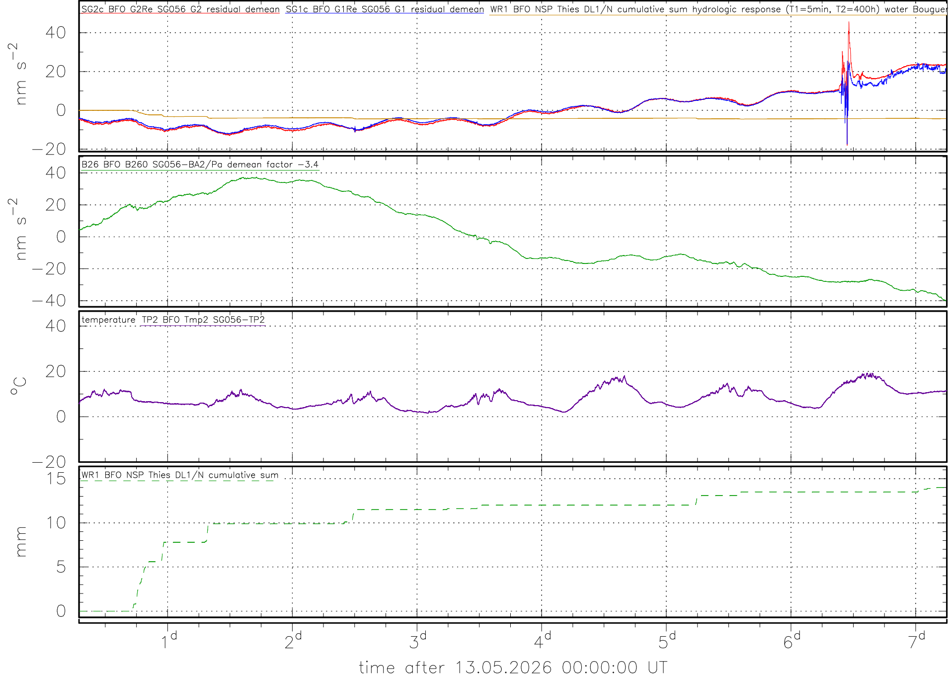
SG056 residuals vs. precipitation (gravity reduced by: drift, tidal model, scaled air-pressure) (plot created at 20.05.2026 06:57:01 UT)
