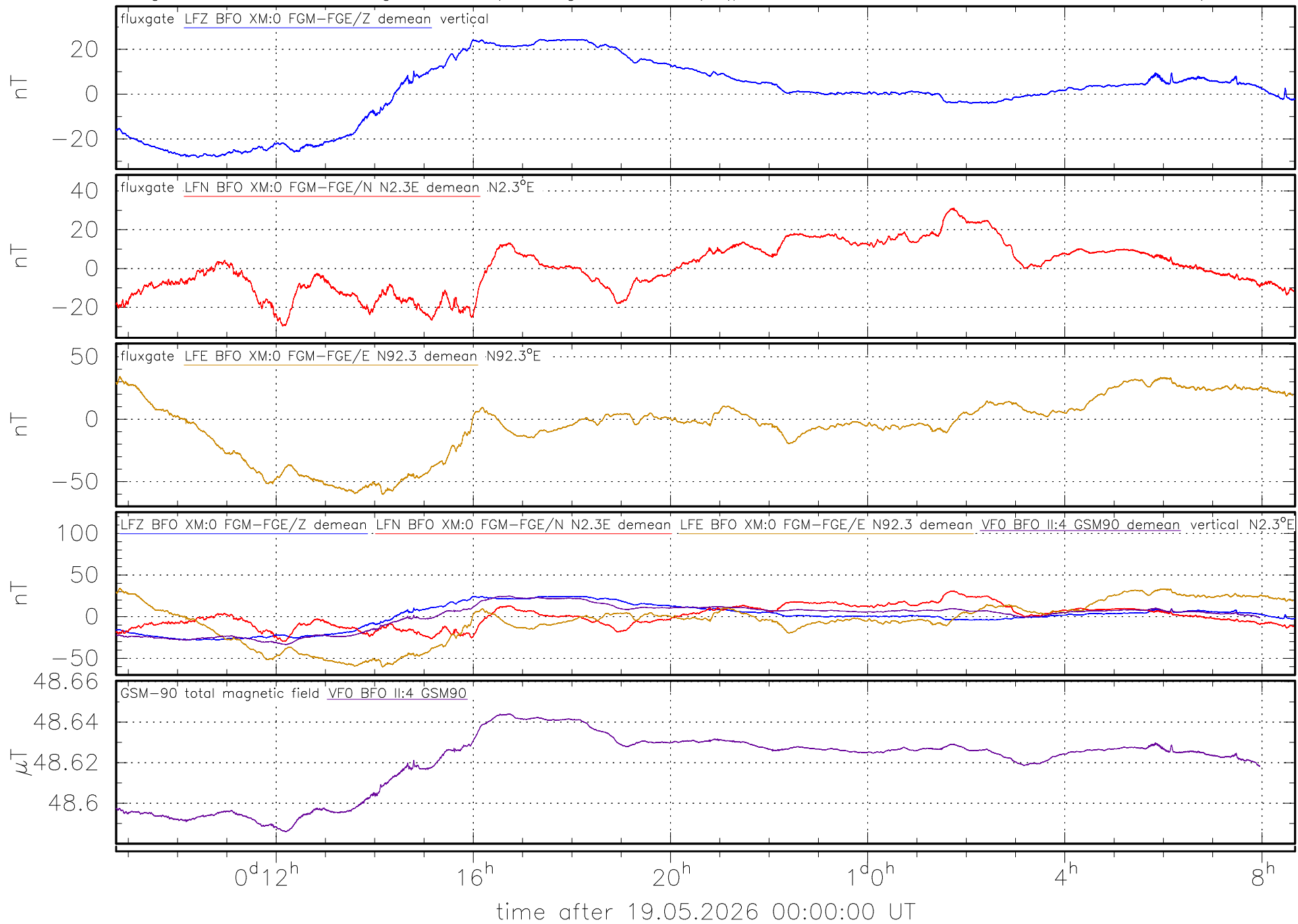
Magnetic field recording @ BFO (average removed) (plot created at 20.05.2026 08:45:17 UT)
