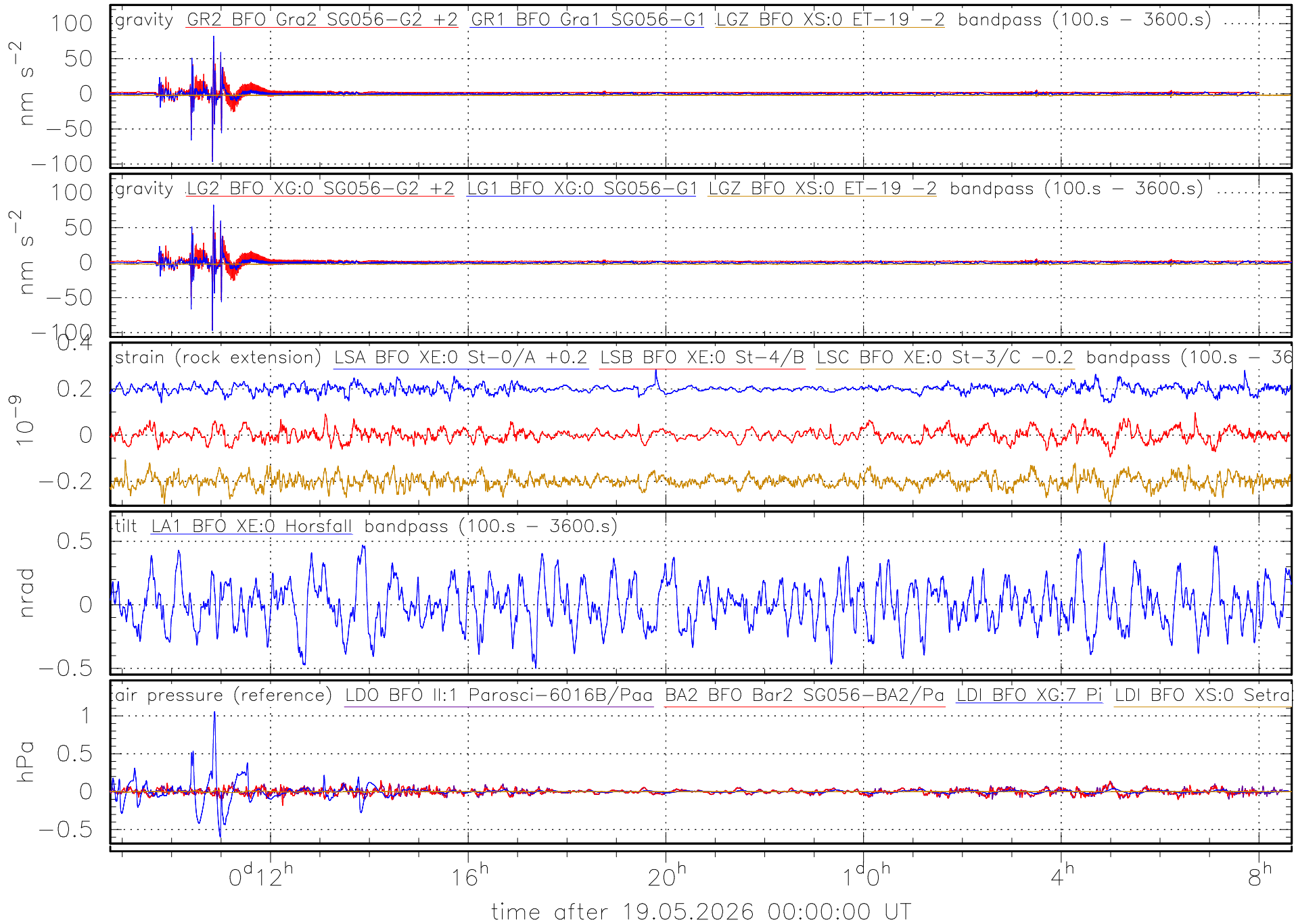
Normal mode bandpass (gravimeters, tilt, strain) (plot created at 20.05.2026 08:45:34 UT)
